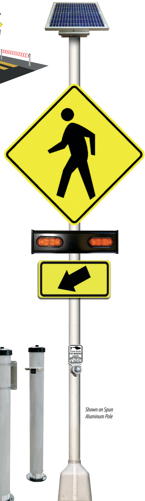
RRFB uses ultra-bright LEDs for maximum visibility
